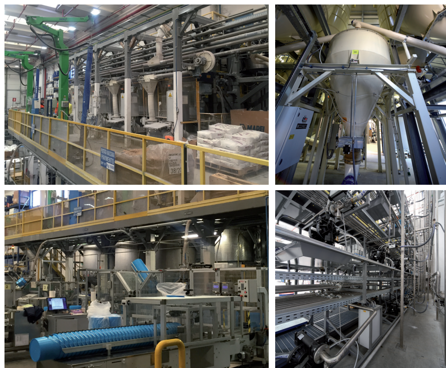
Figure 1: production process - © Photo Halvor Gudim
