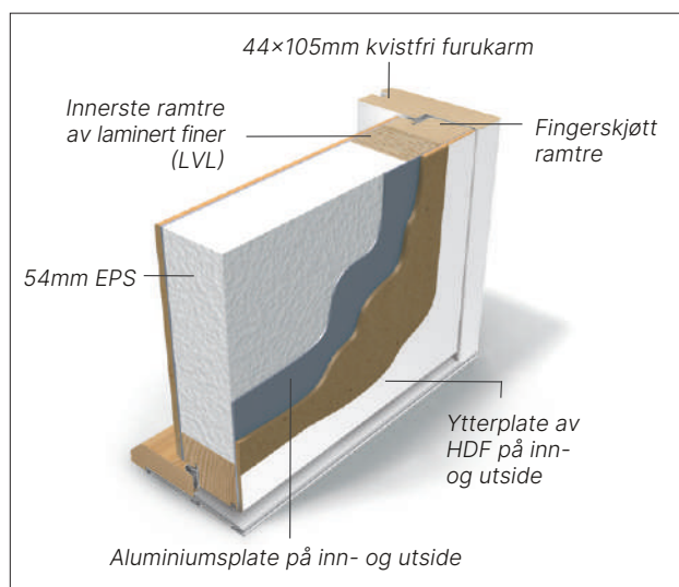
Snitt YD STD
