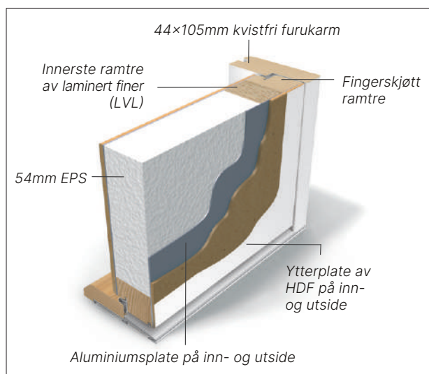
Snitt YD Prisgunstig
